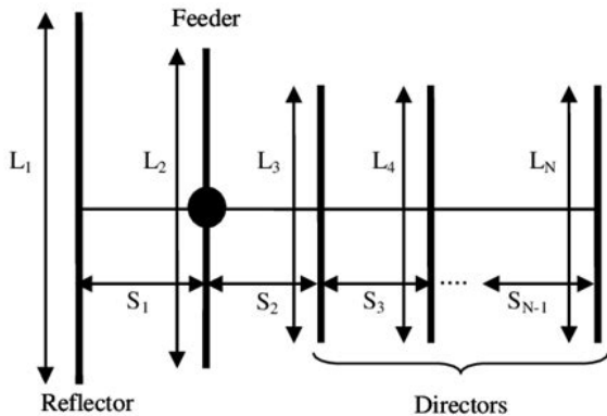
Figure 3: Yagi antenna
