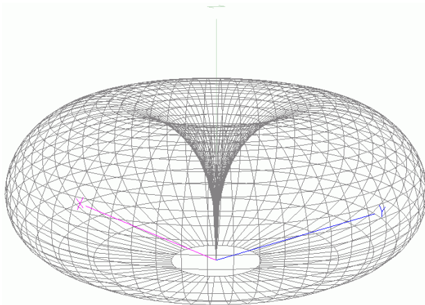
Figure 5: Monopole polarization
